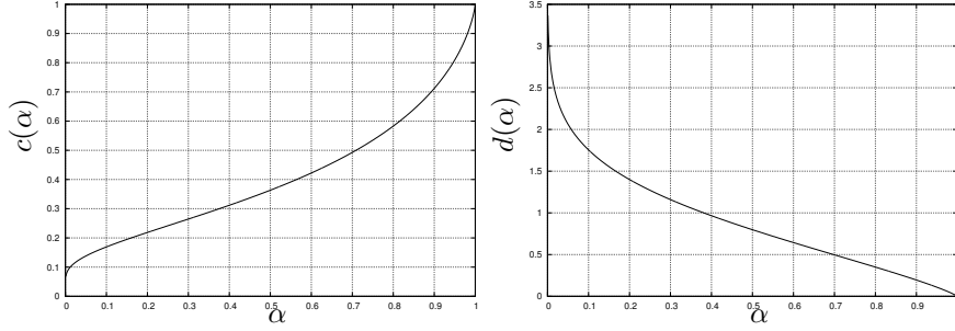
Figure 2: Illustration of c(\alpha) and d(\alpha)
