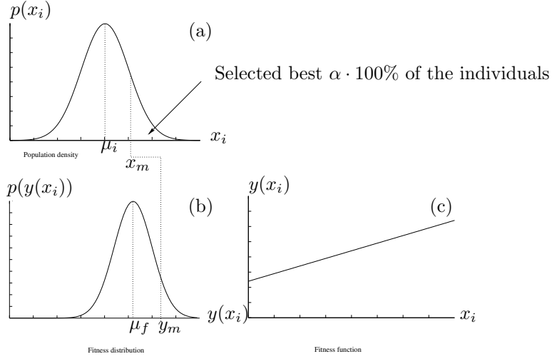
Figure 1: Impact of truncation selection of the best \alpha \cdot 100\% individuals on the fitness distribution (b) and the population density (a). We assume an increasing fitness function (c). The fitness distribution is truncated from the left in y_m . The population distribution is truncated from the left in the corresponding point x_m .
